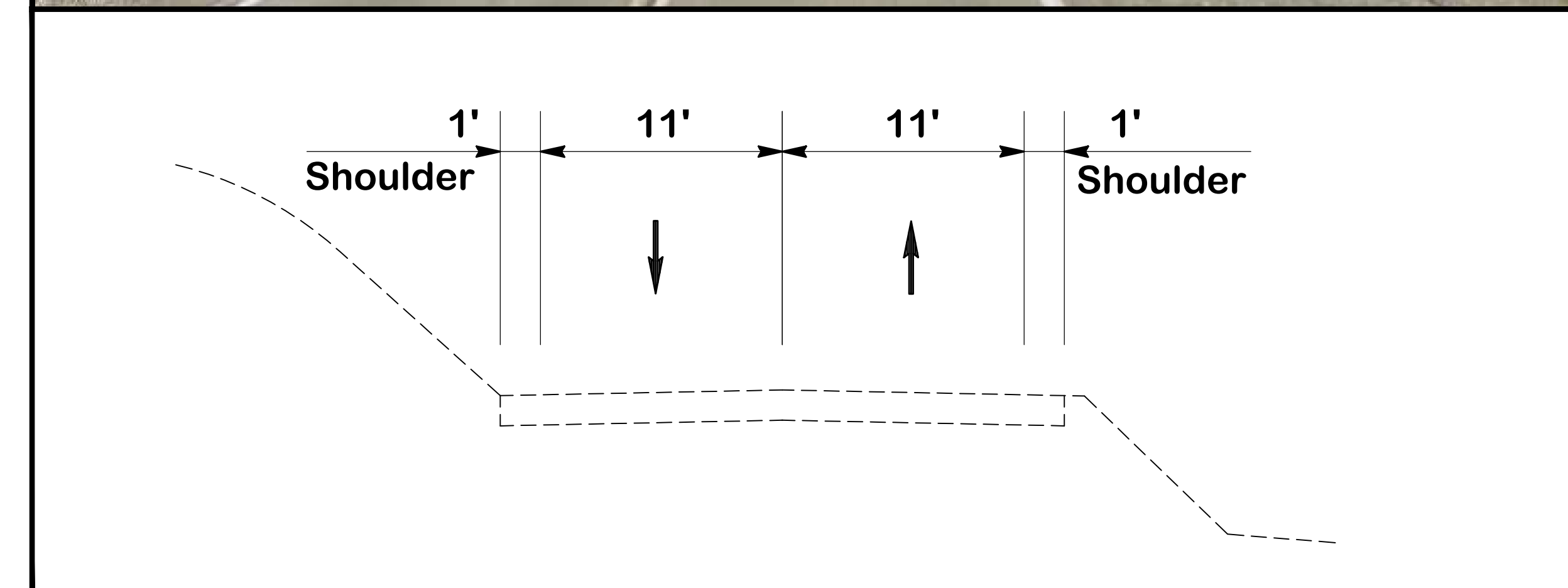
SECTION I-I NO SCALE
