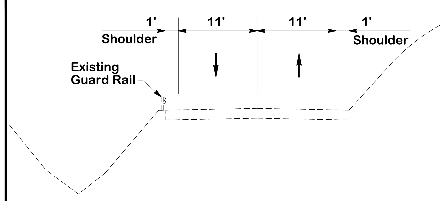
SECTION F-F NO SCALE
