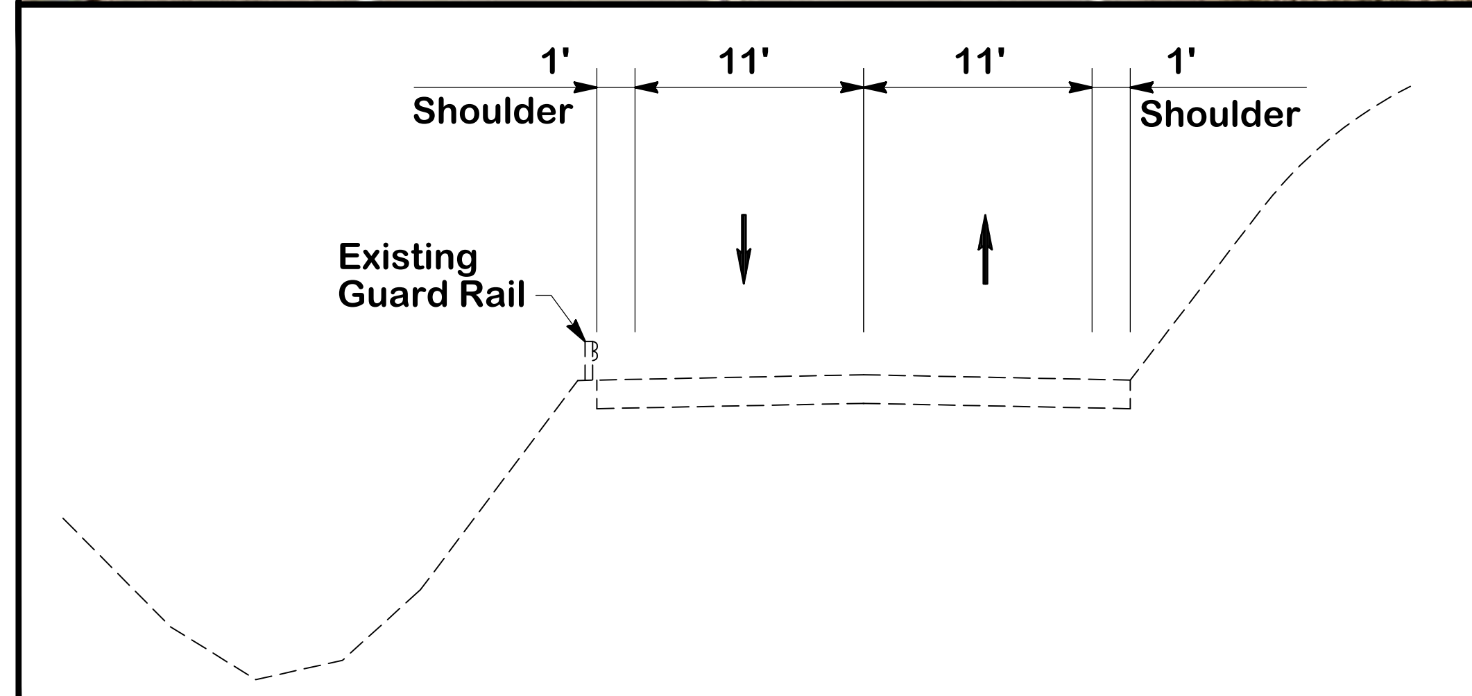
SECTION G-G NO SCALE
