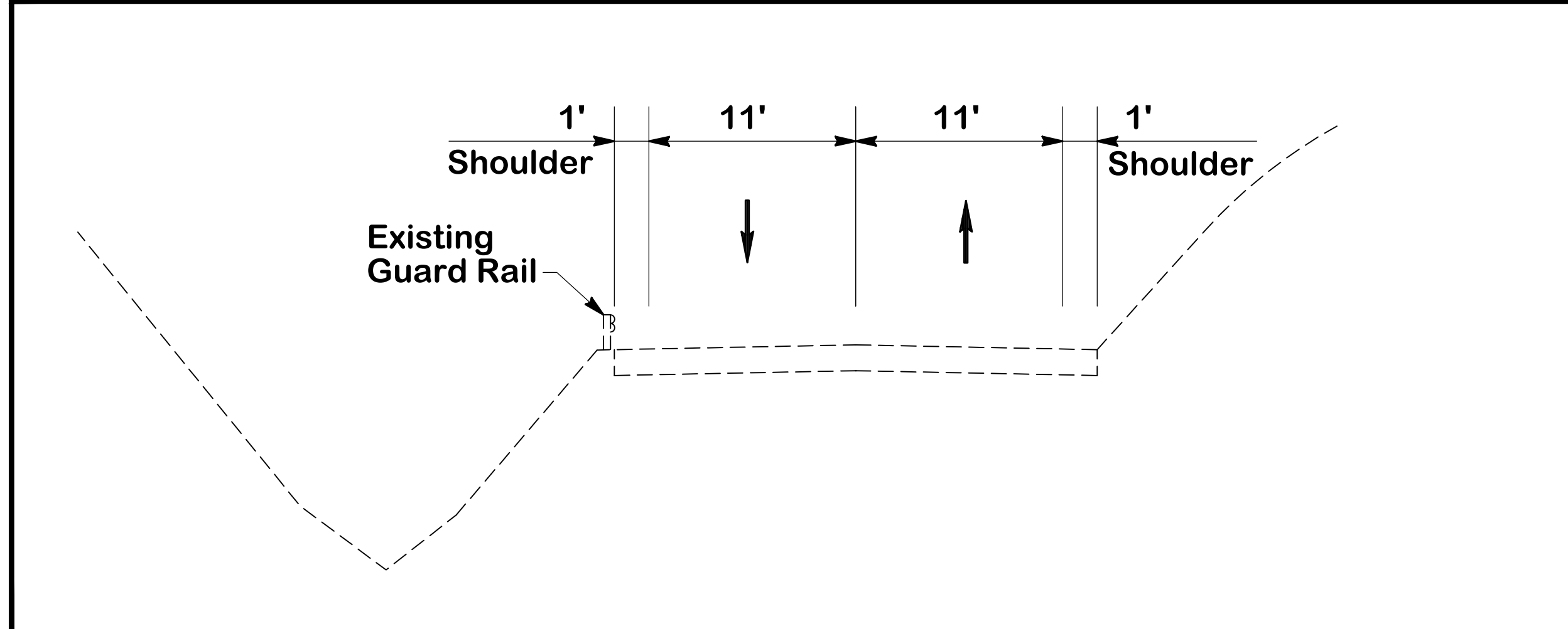
SECTION H-H NO SCALE
