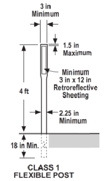
DELINEATOR DETAIL NOT TO SCALE
